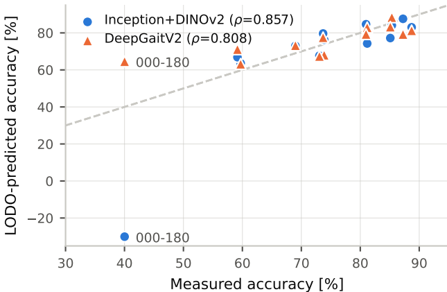
(a) From scratch
