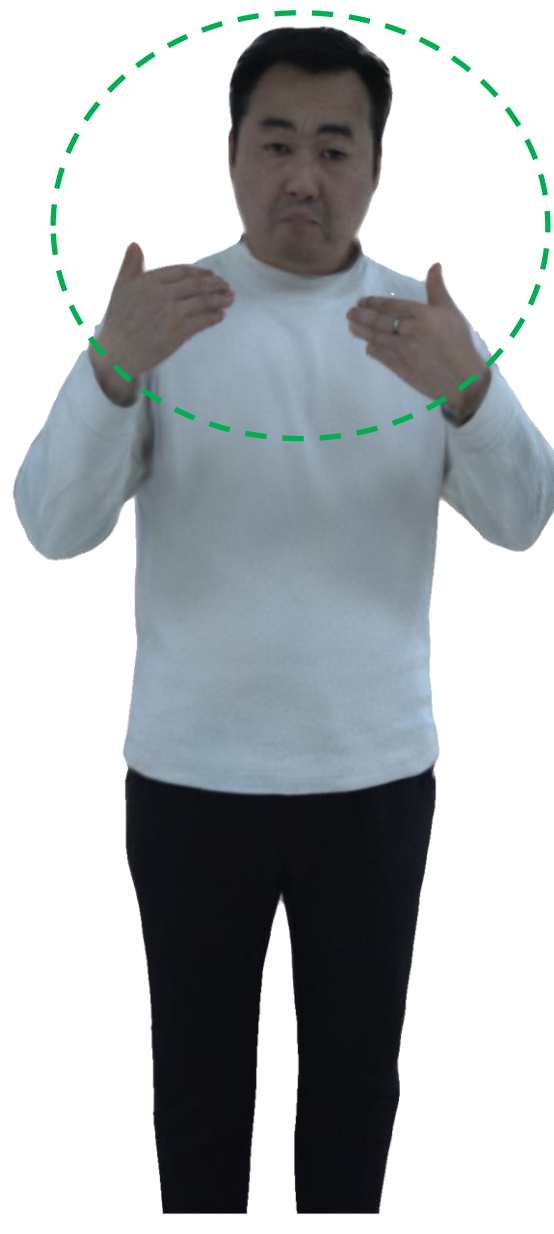
Combine
