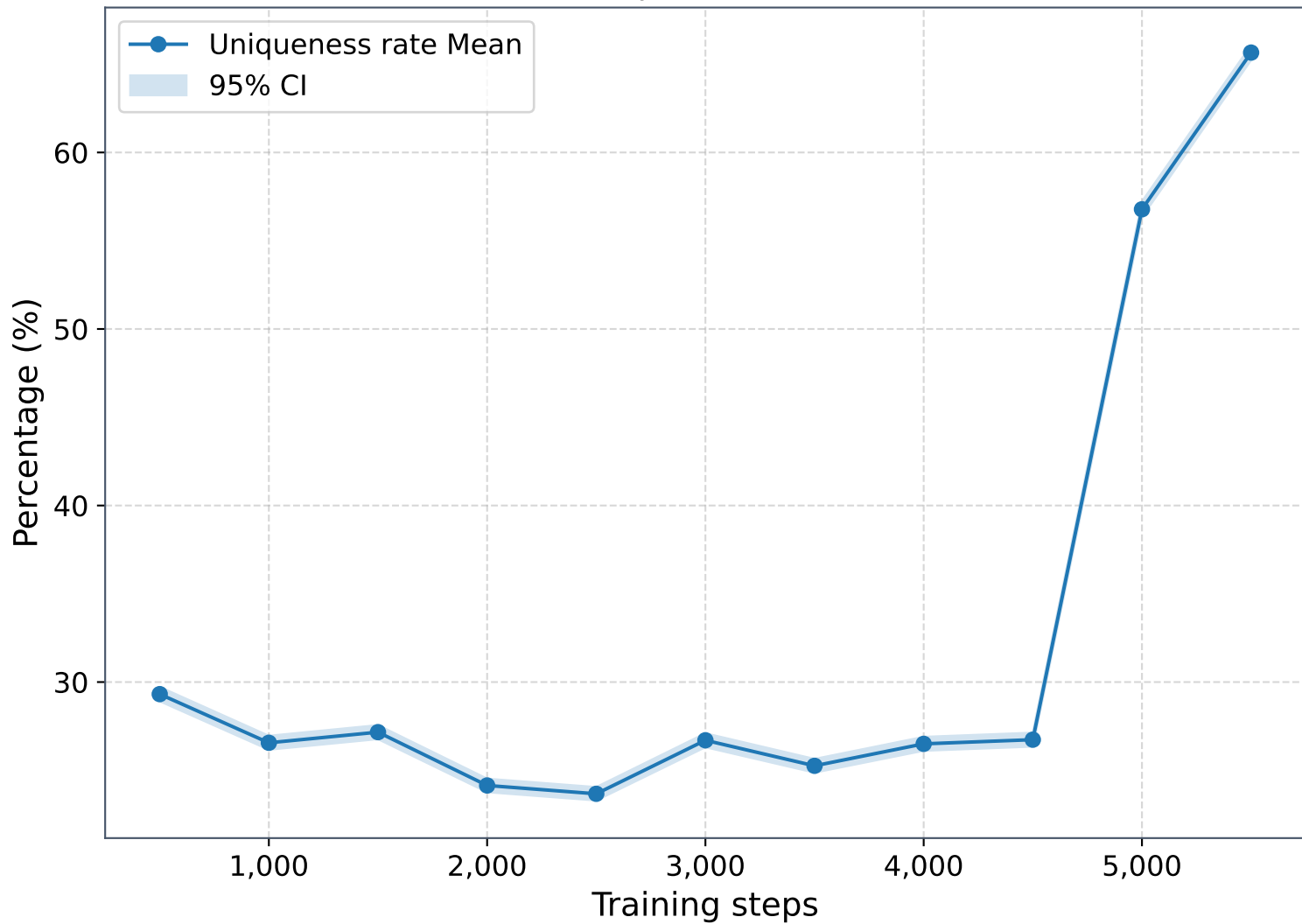
Uniqueness rate
