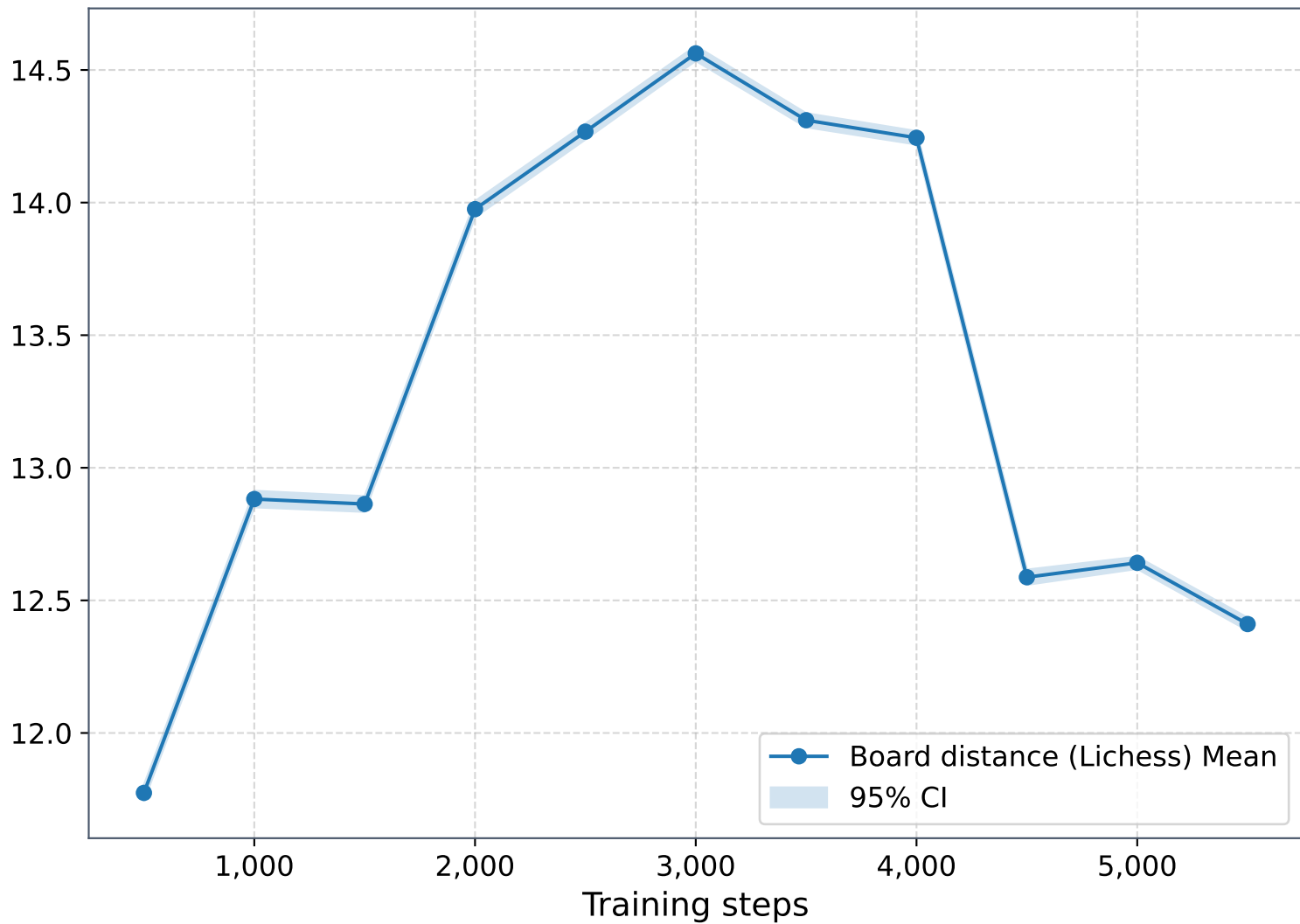
Board distance (Lichess)
