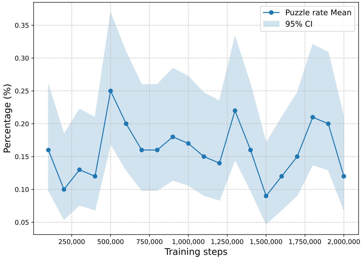
Puzzle rate
