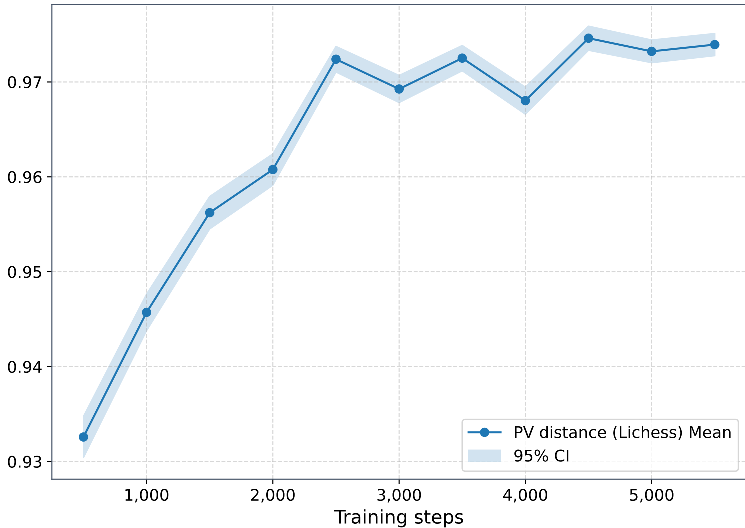
PV distance (Lichess)
