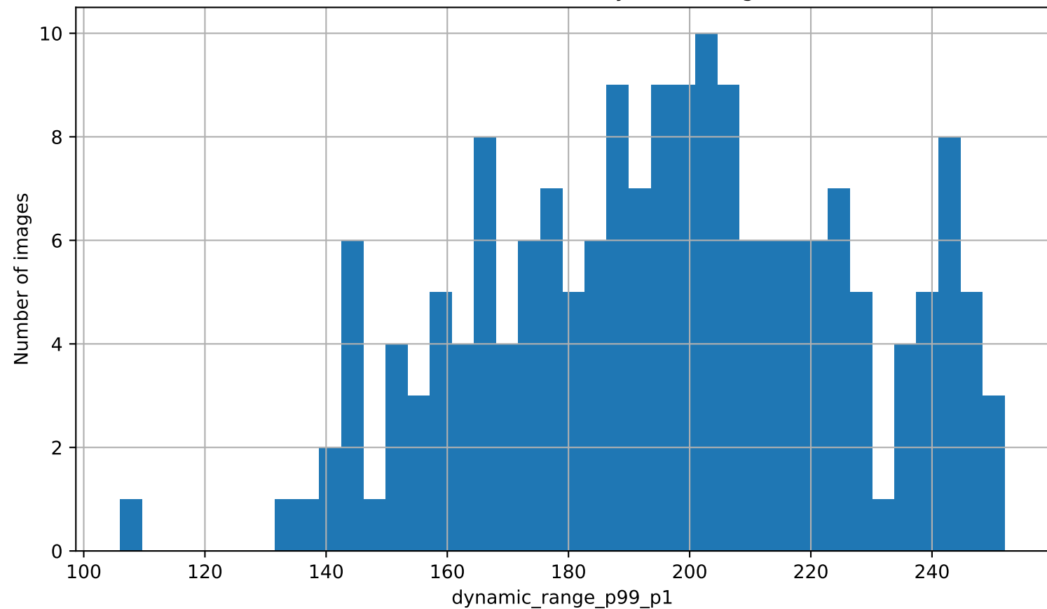
Distribution of robust dynamic range
