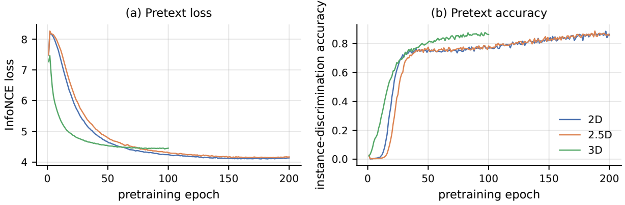
Figure 3: MoCo v2 pretext training on the 5133-nodule pool. All three encoders learn the pretext task; 3D uses a 100-epoch schedule.
