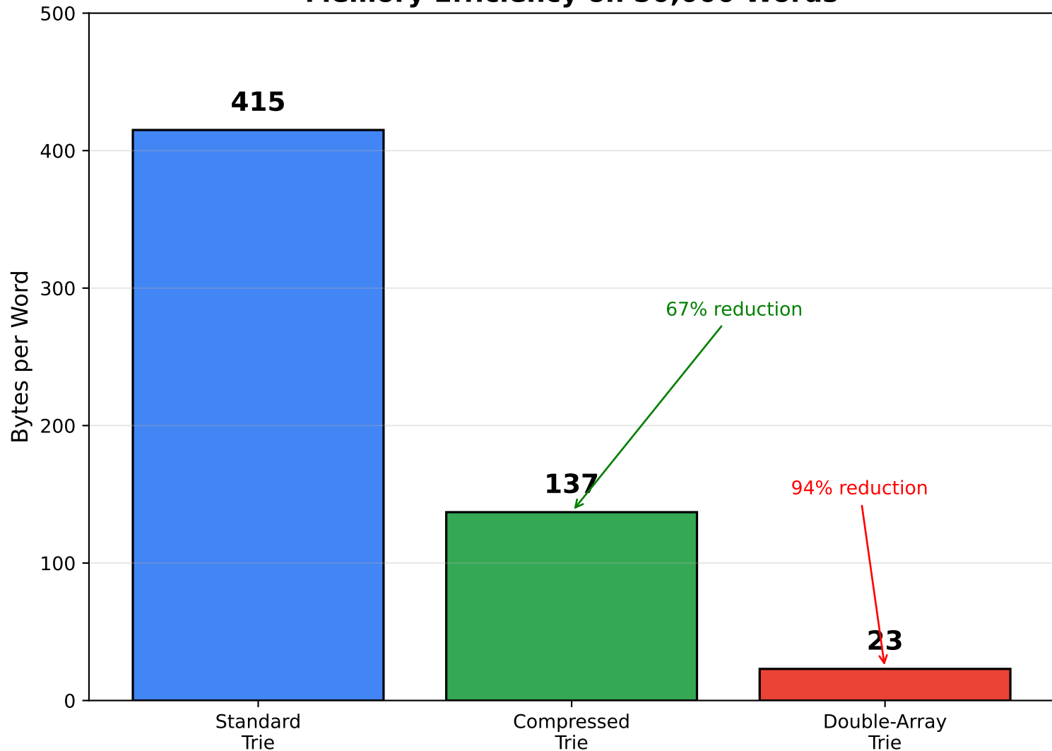
Memory Efficiency on 50,000 Words
