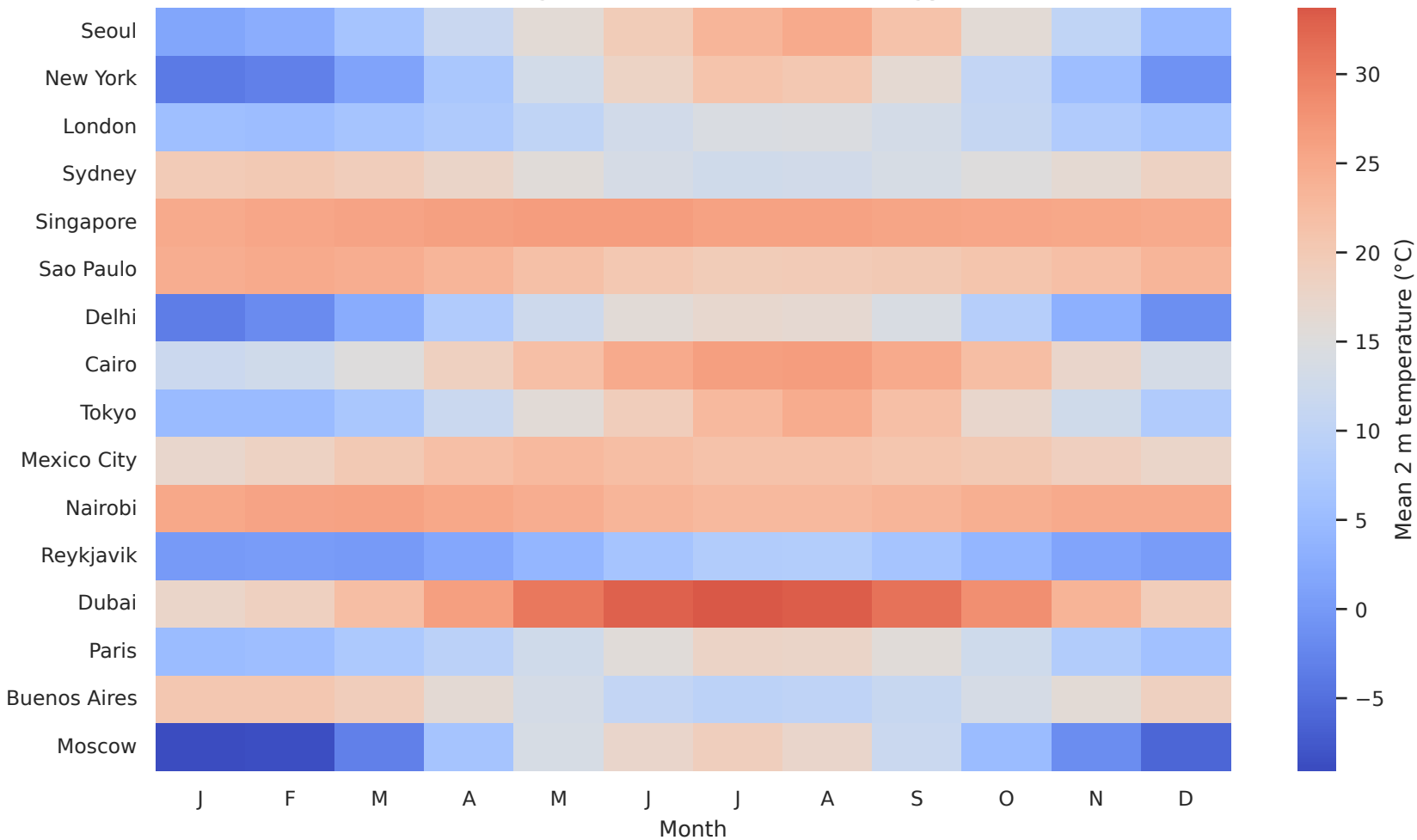
Training-period seasonal climatology
