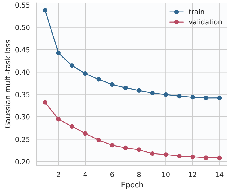
Optimization convergence
