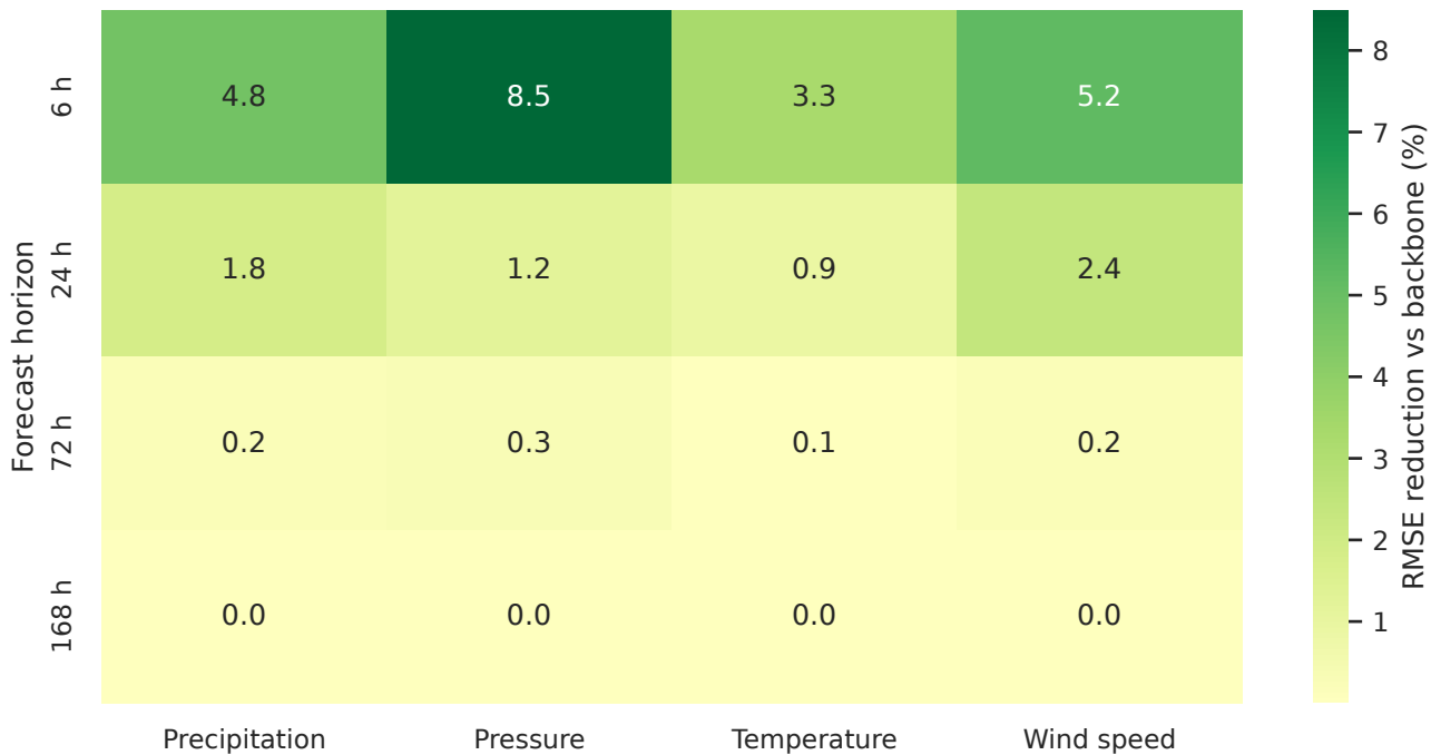
Where persistent retrieval improves the neural backbone
