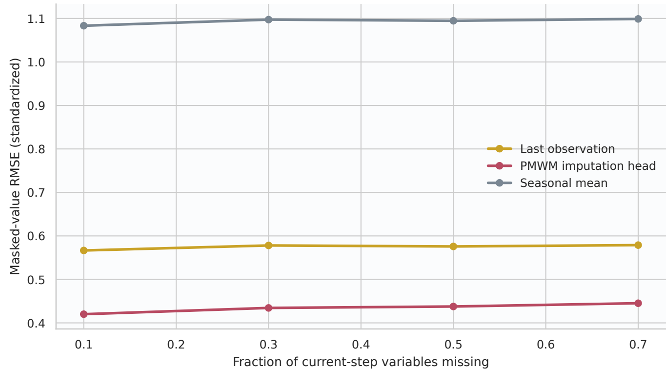
Robust current-step imputation under increasing missingness
