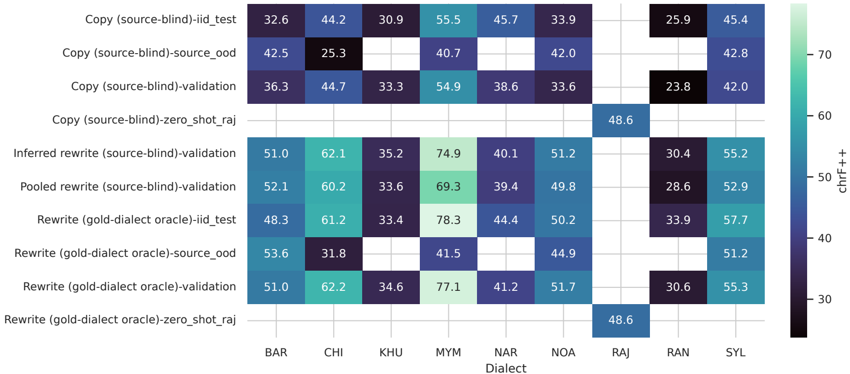
Source-blind controls and disclosed gold-dialect oracle
