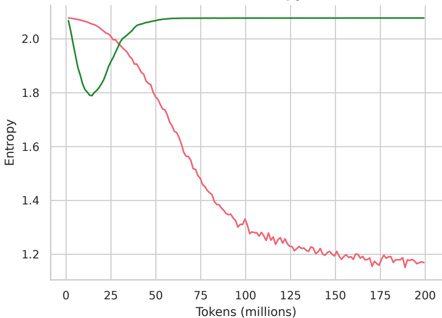
Router entropy
