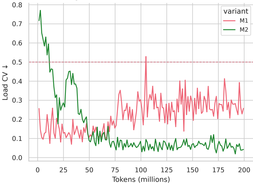
Expert-load coefficient of variation
