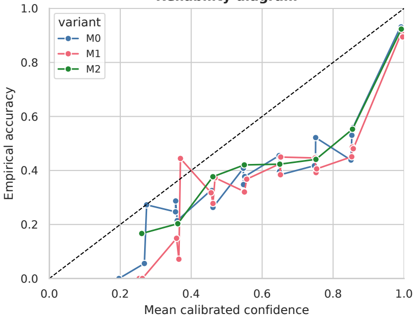
Reliability diagram
