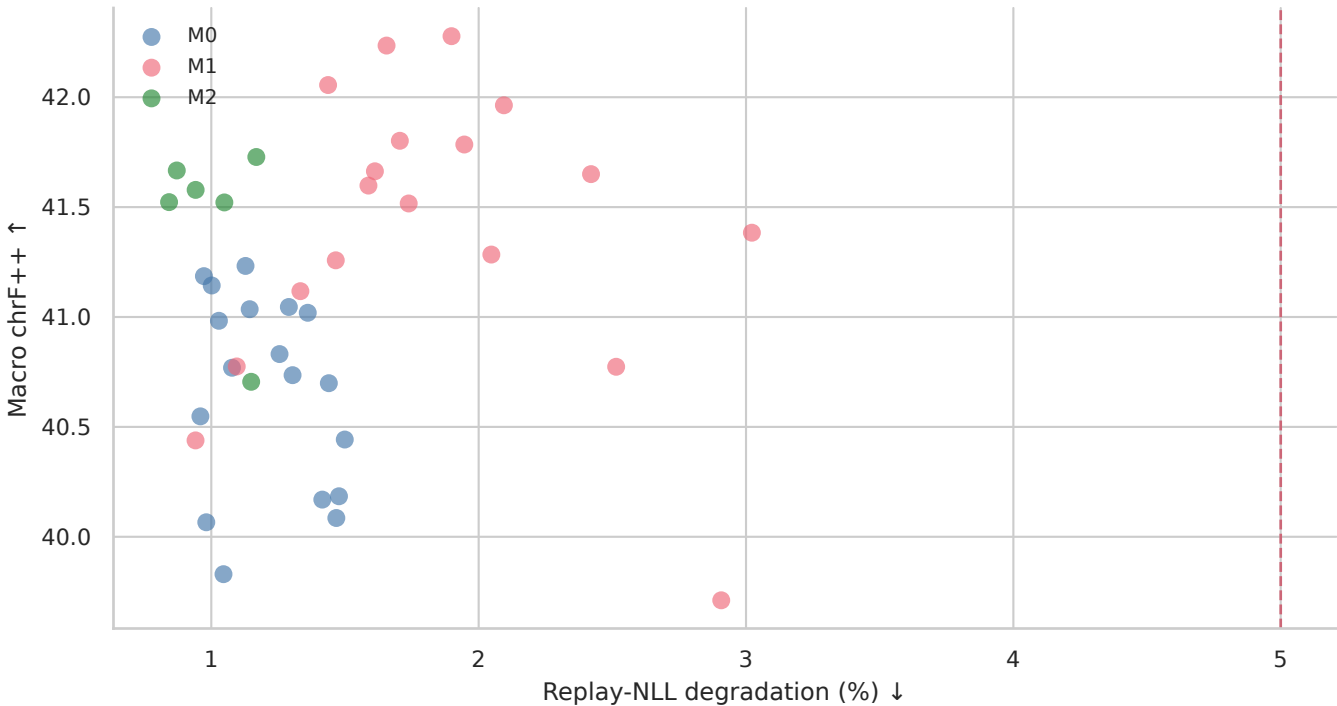
Main-run task quality under the retention guard
