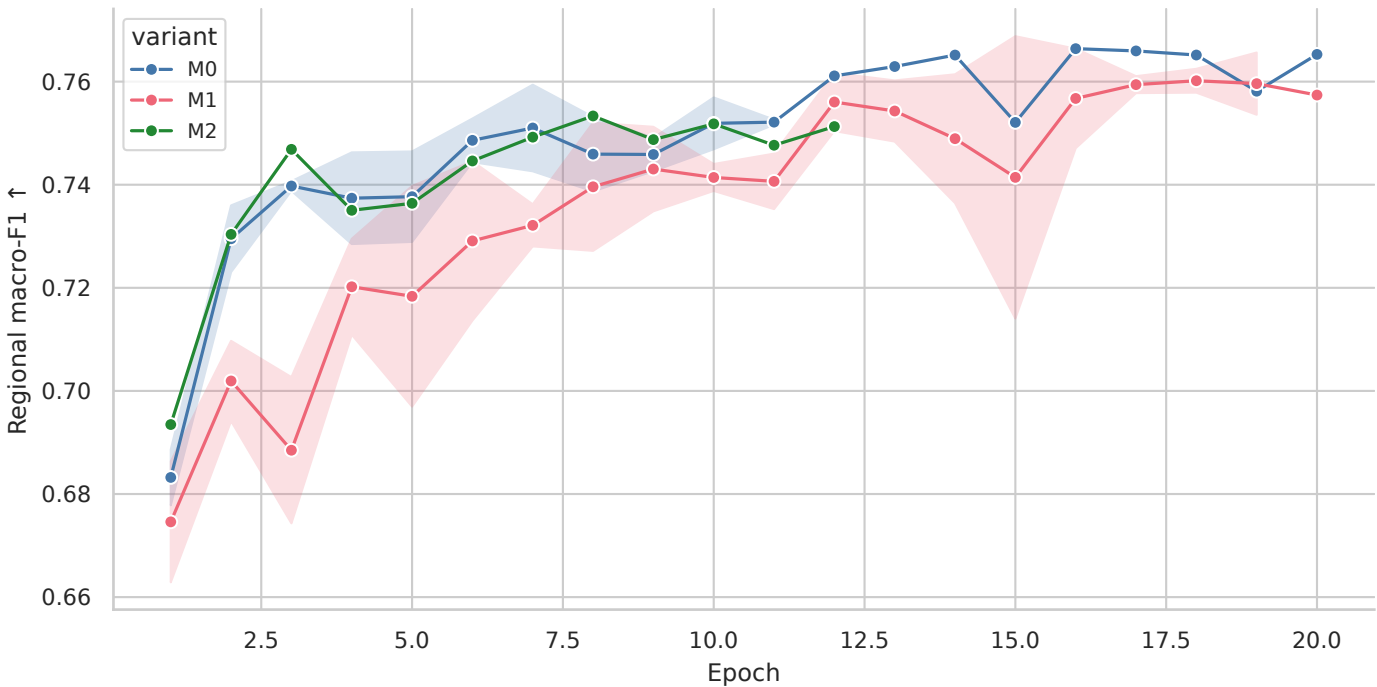
Causal identification validation trajectories
