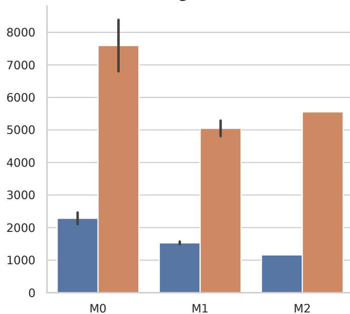
Training tokens/s ↑
