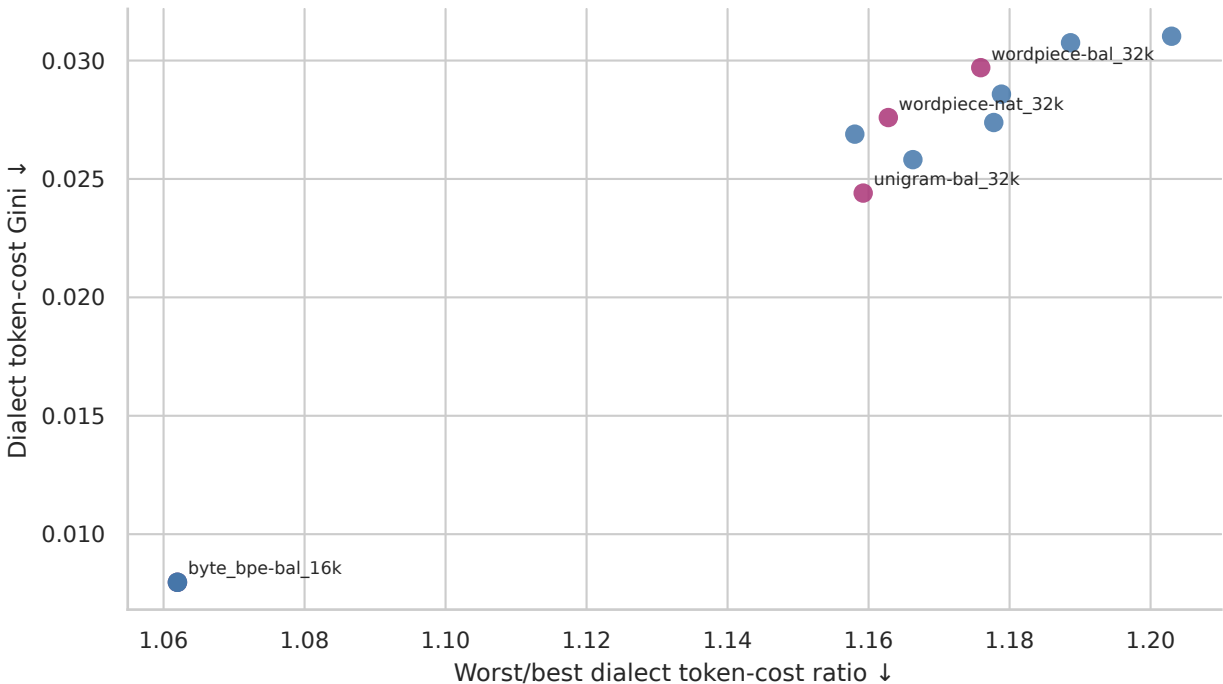
Tokenizer parity across dialects
