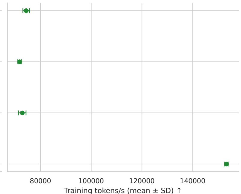
Proxy throughput
