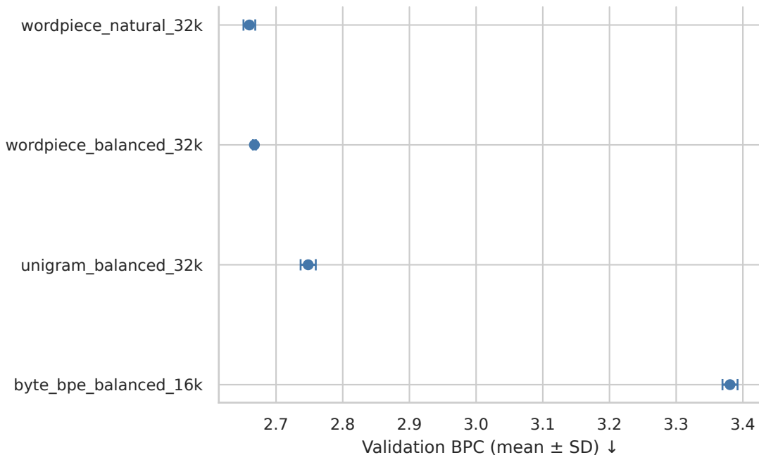
Three-seed proxy quality
