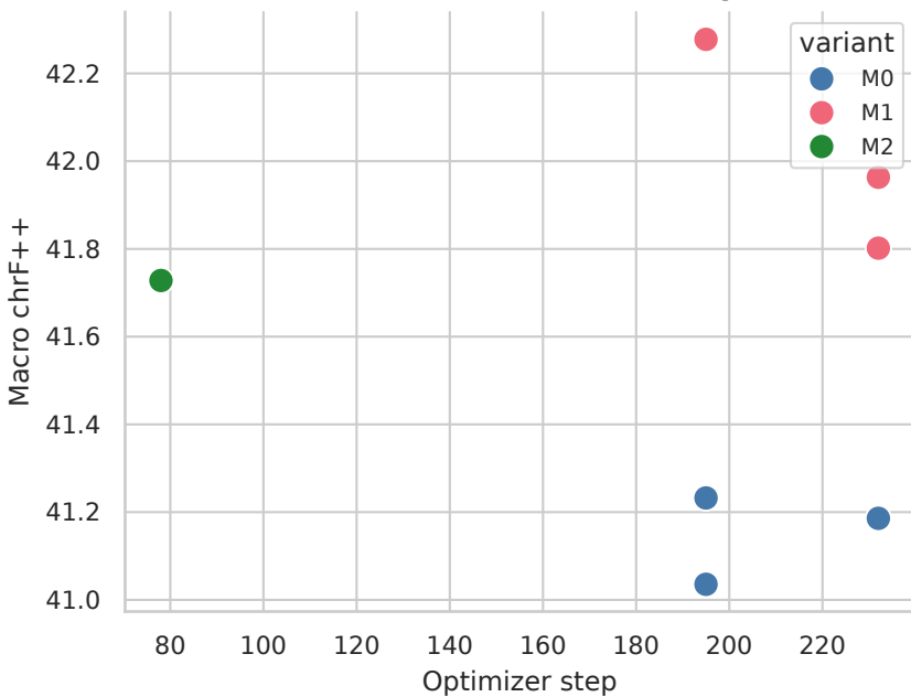
Selected normalization checkpoint
