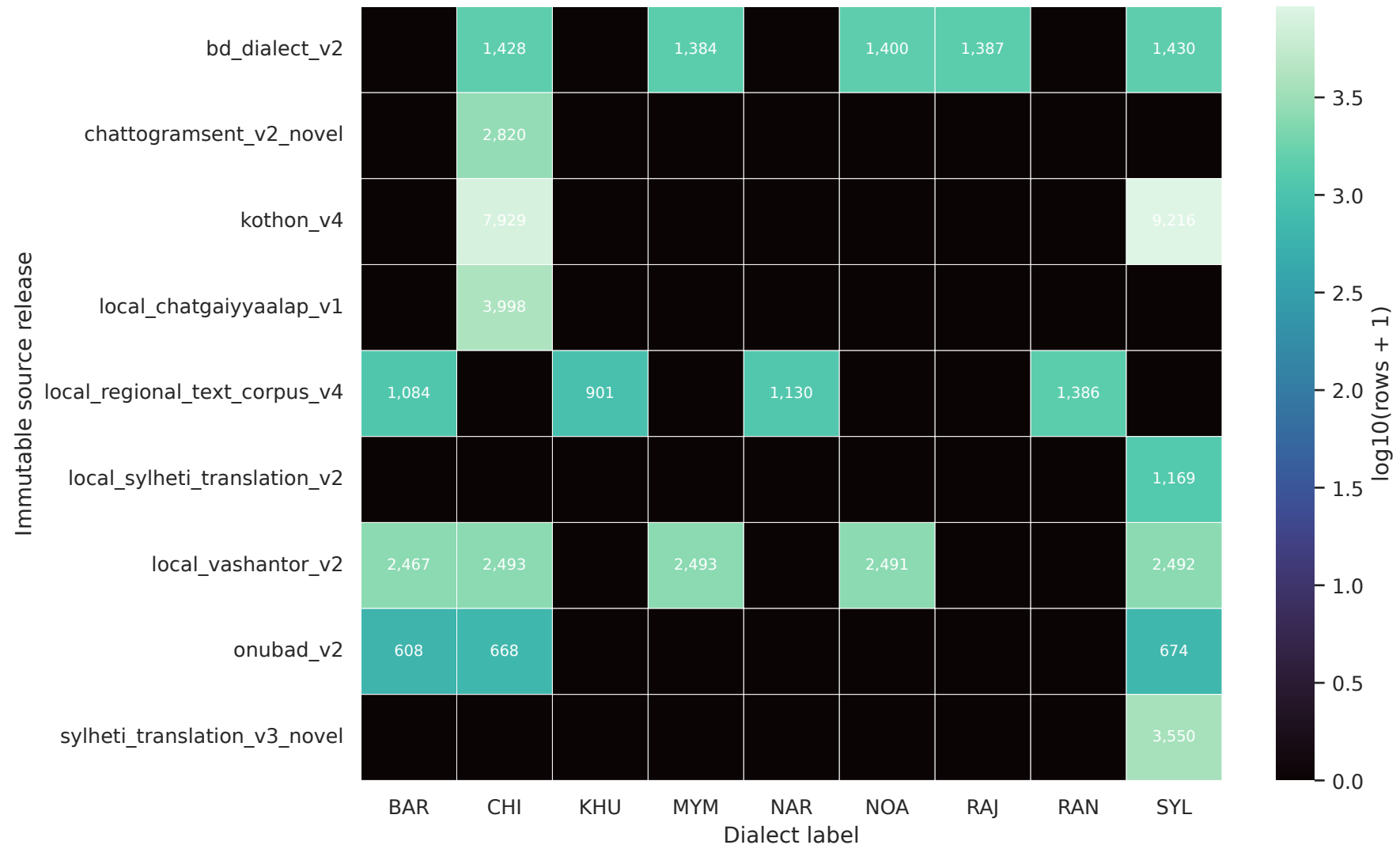
Authentic normalization coverage by source and dialect
