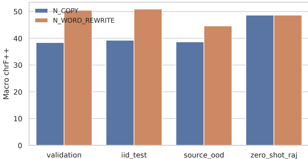
Non-neural normalization floors
