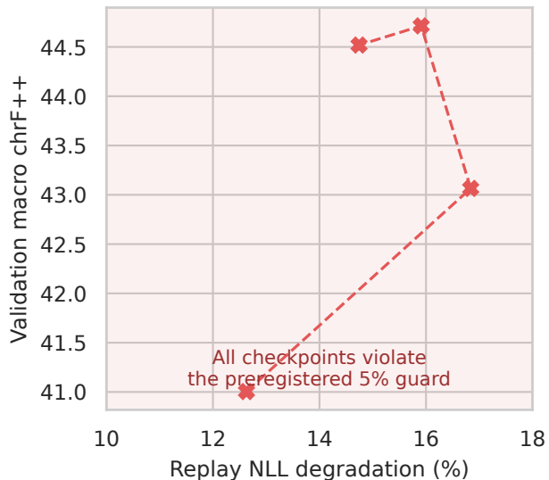
Original schedule: task gain with forgetting
