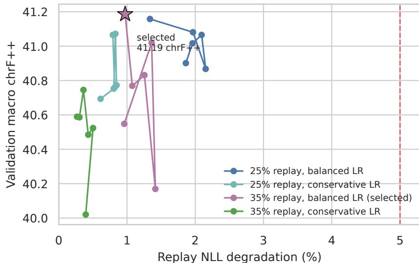
Registered replay-safe schedules
