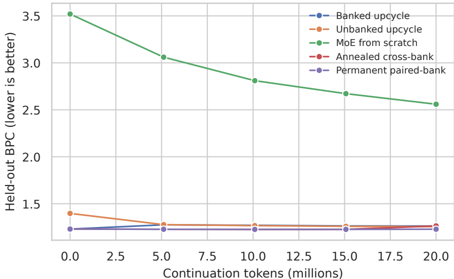
Development-only dense→MoE recovery pilot
