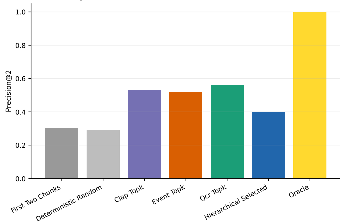
Evaluation precision@2
