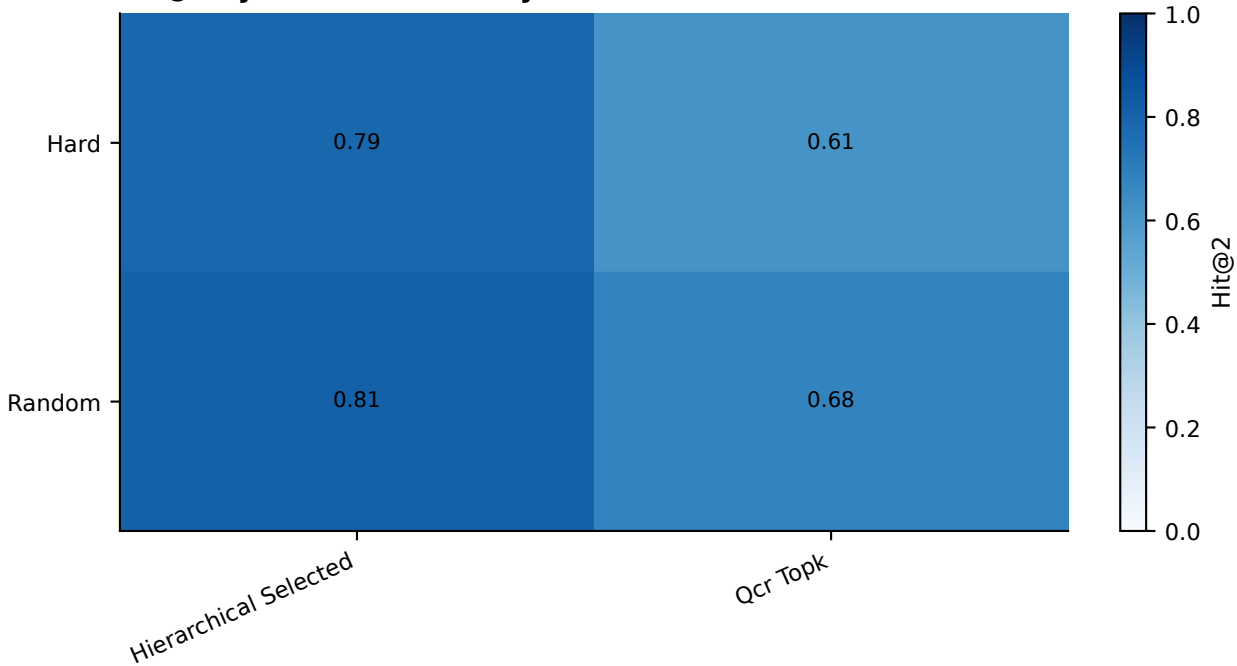
Hit@2 by retrieval difficulty
