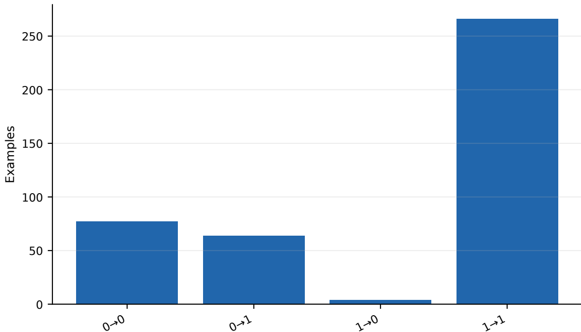
Example-level Hit@2 transitions
