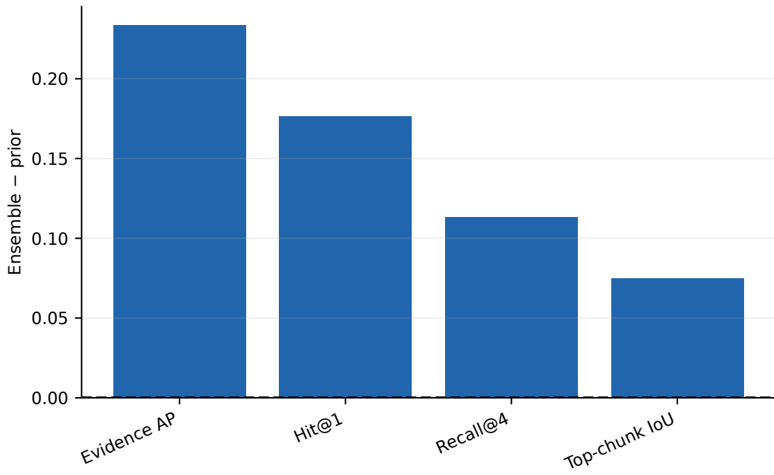
Absolute gain over frozen CLAP prior
