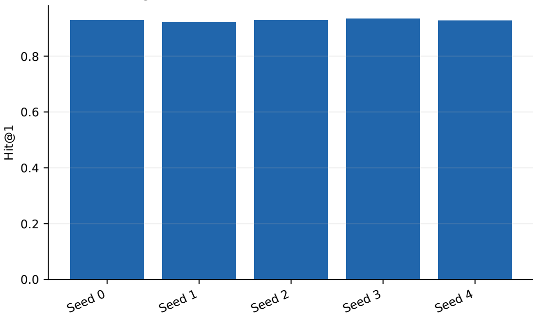
Per-seed Hit@1
