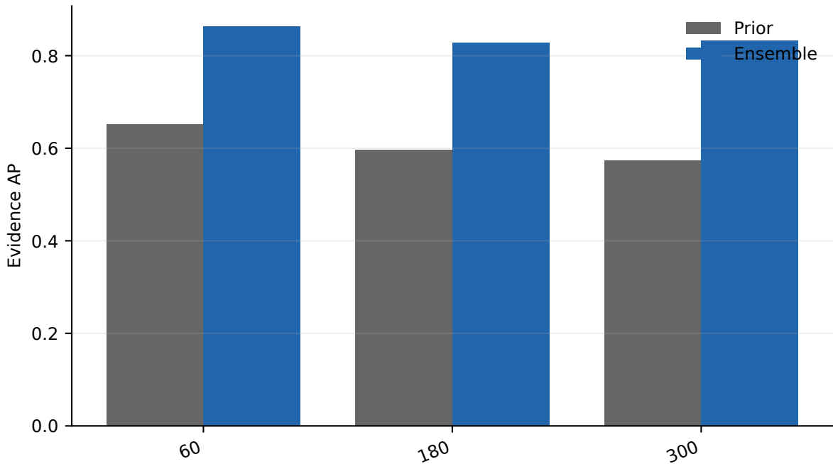
Evidence AP by Duration (s)
