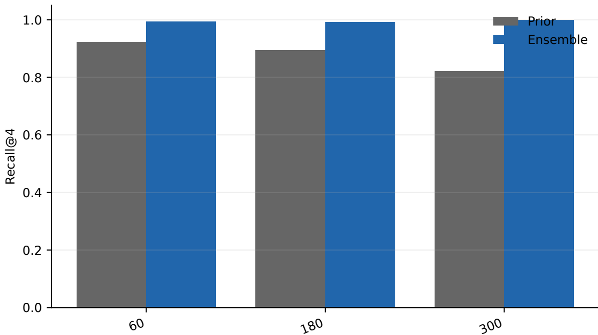
Recall@4 by Duration (s)
