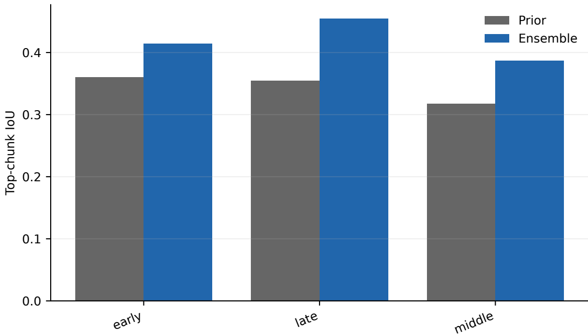
Top-chunk IoU by Target position
