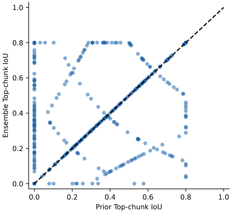
Per-example IoU transfer
