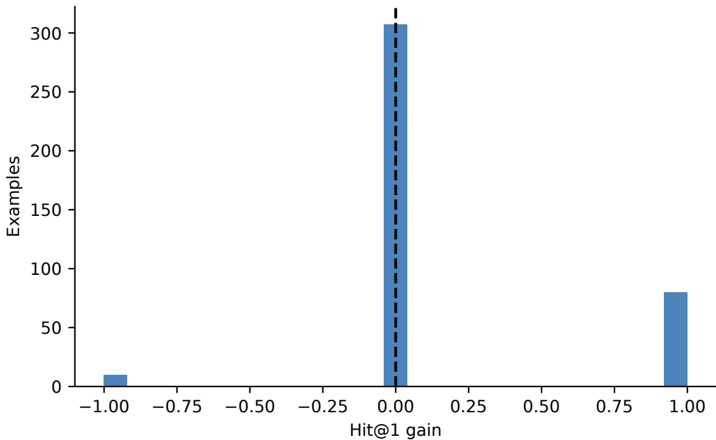
Per-example Hit@1 gain distribution
