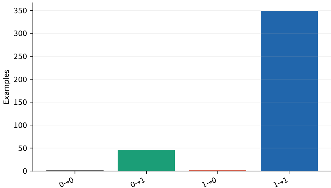
Recall@4 transition
