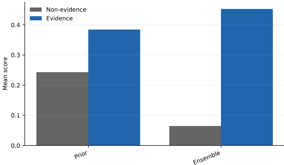
Evidence/non-evidence score separation
