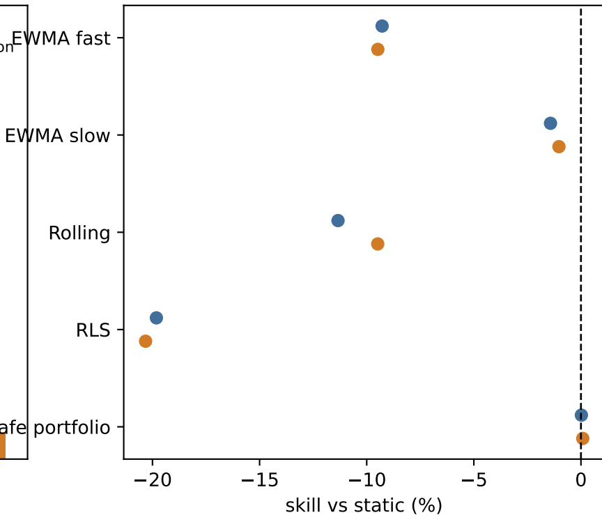
Unconstrained-adapter ablation
