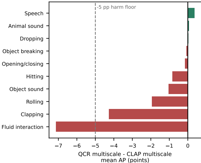
Classwise transfer on natural audio
