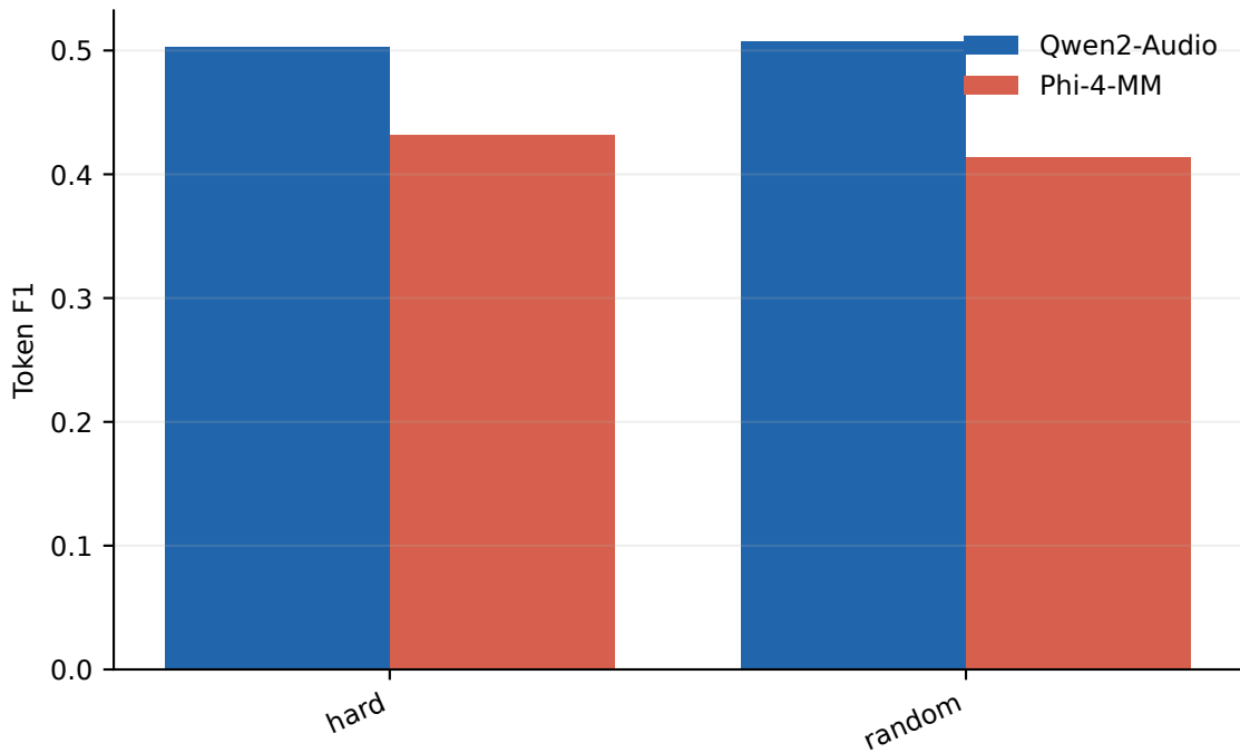
Selected-system token f1 by difficulty
