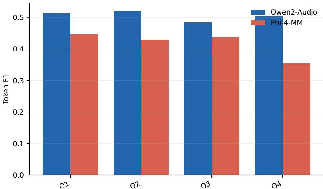
Selected-system token f1 by chunk-count quartile
