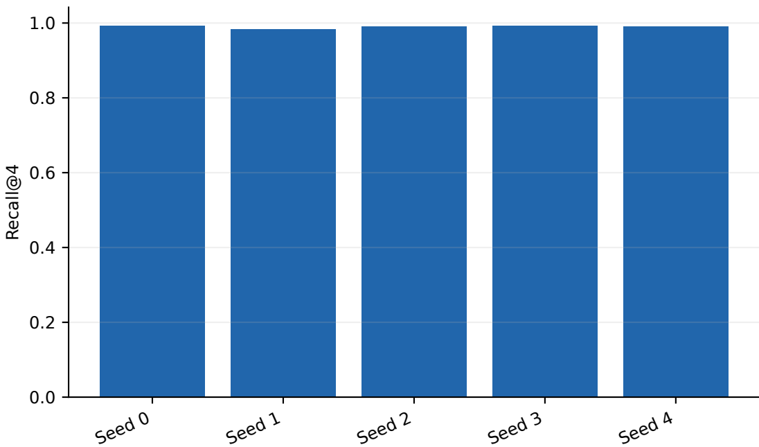
Per-seed Recall@4
