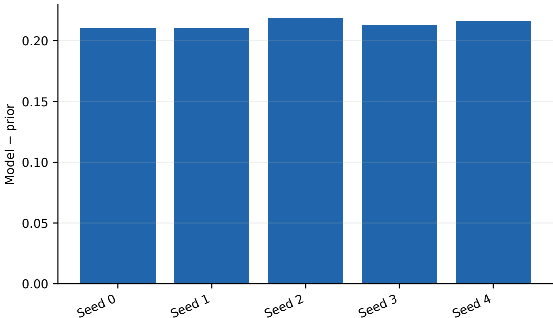
Per-seed Evidence AP gain
