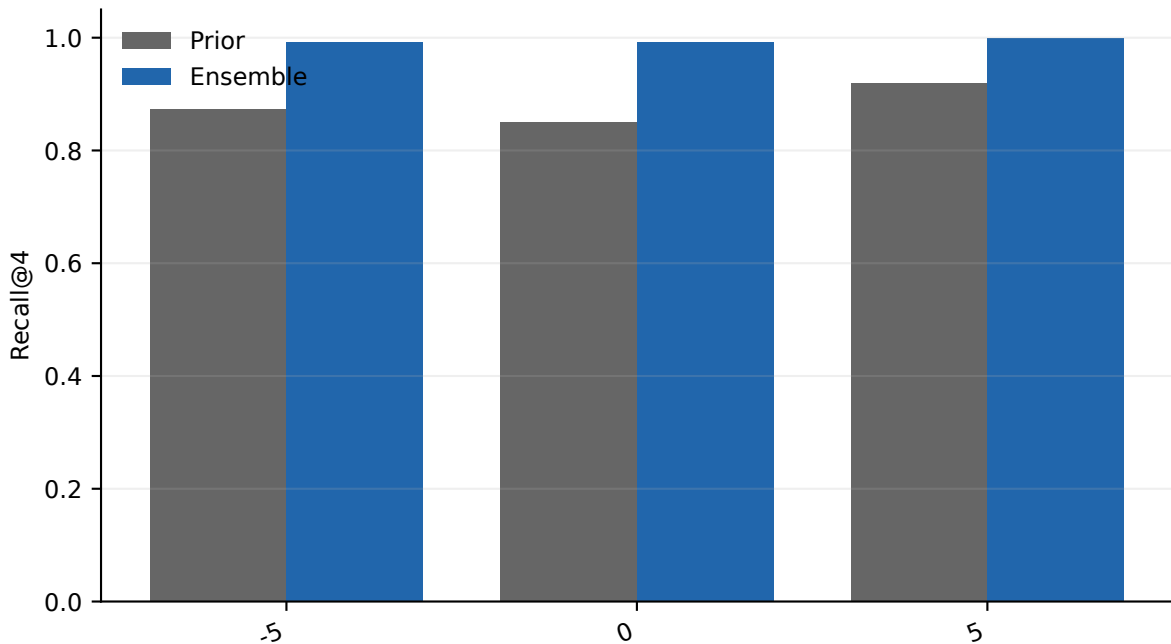
Recall@4 by SNR (dB)
