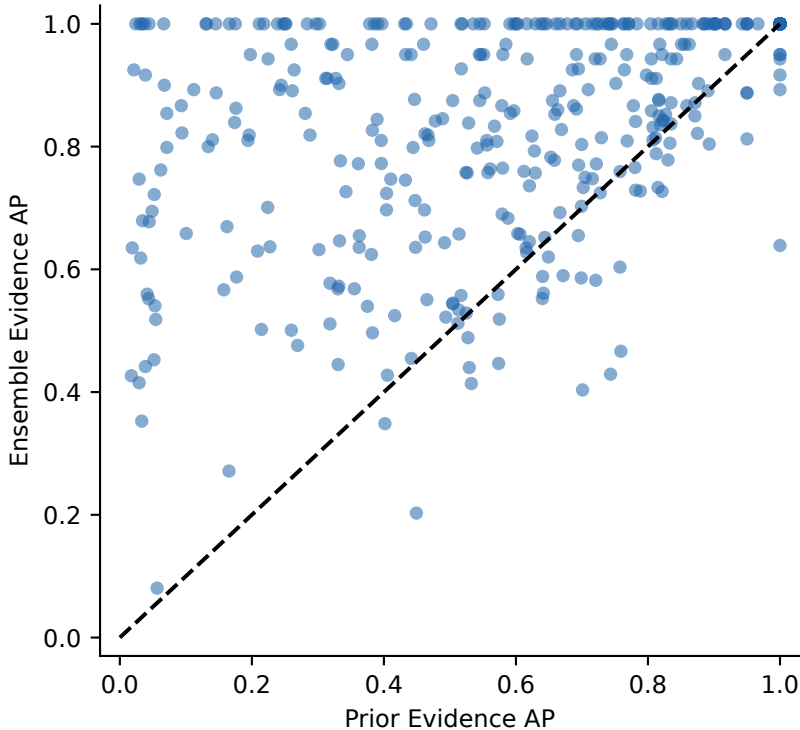
Per-example AP transfer
