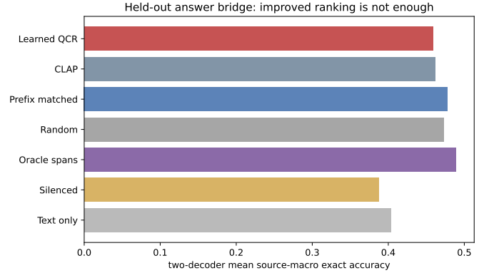
Fig. 1. Two-decoder mean source-macro exact answer accuracy. Oracle spans are context, not an eligible learned comparator.
