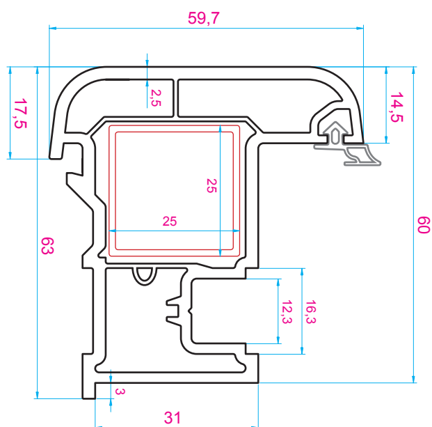
6040A-40 - 959 gr/m / Profil Adaptor Aripa - Mullion Rebate Profile
