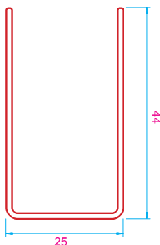
Profil Usa Interior - Profil Usa Exterior Door Sash Profile Outside Opening Door Sash Profile
