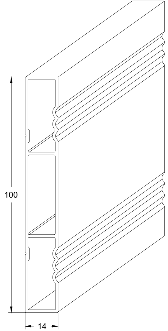
Çit Panel Profili PANELLING PROFILE
