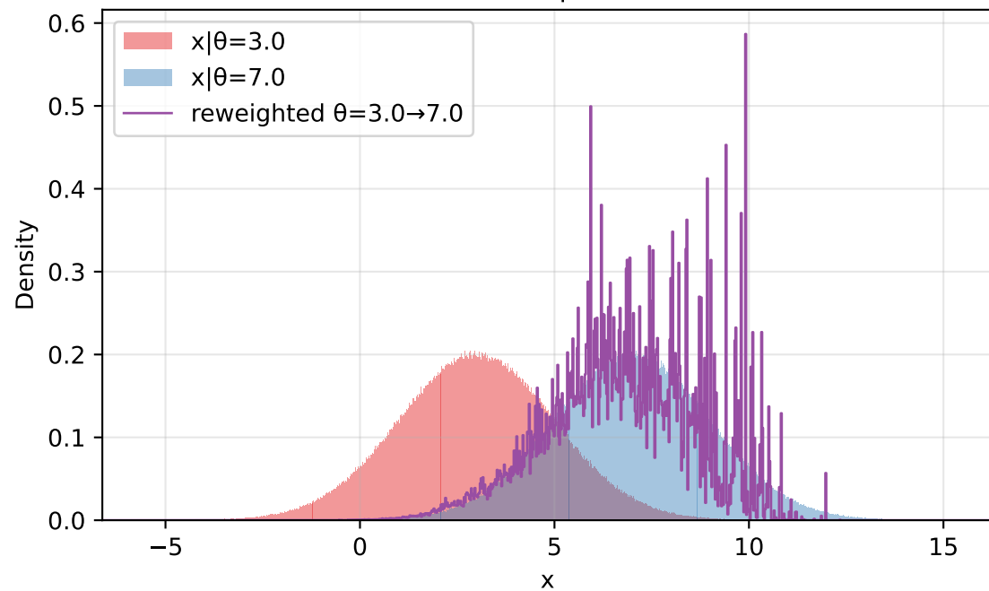
grid prior N=1,000,000 | ESS=1,111
