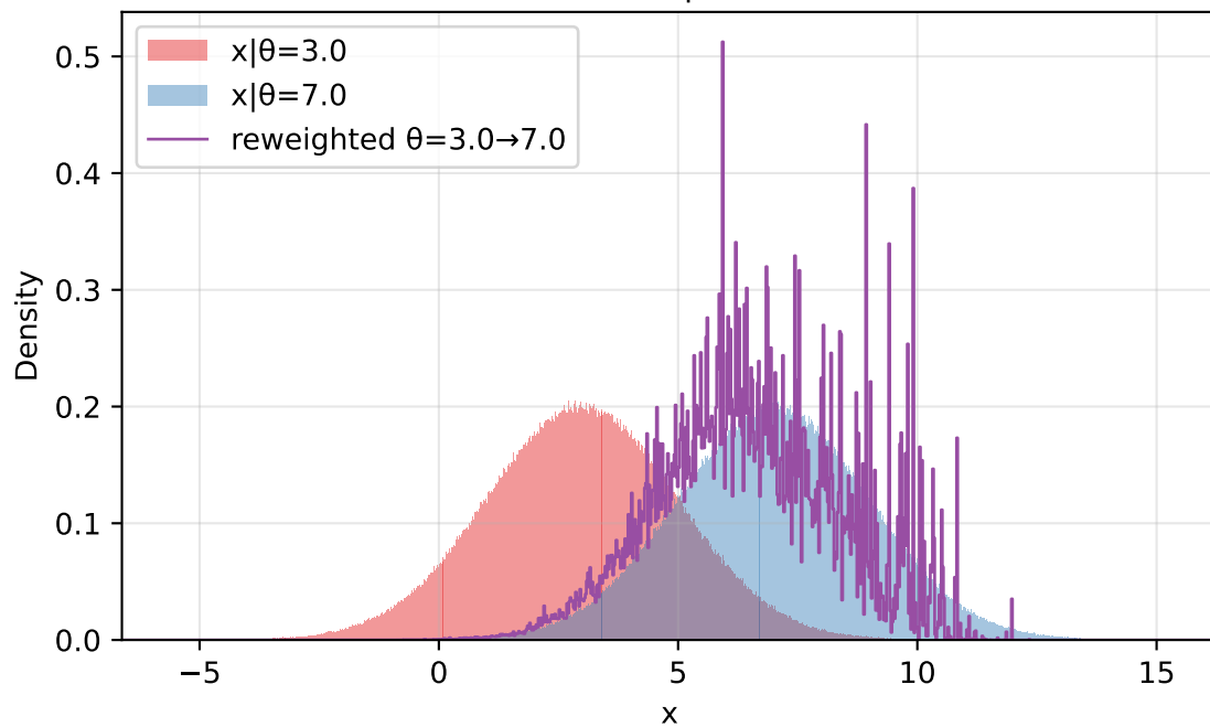
exponential prior N=1,000,000 | ESS=1,548
